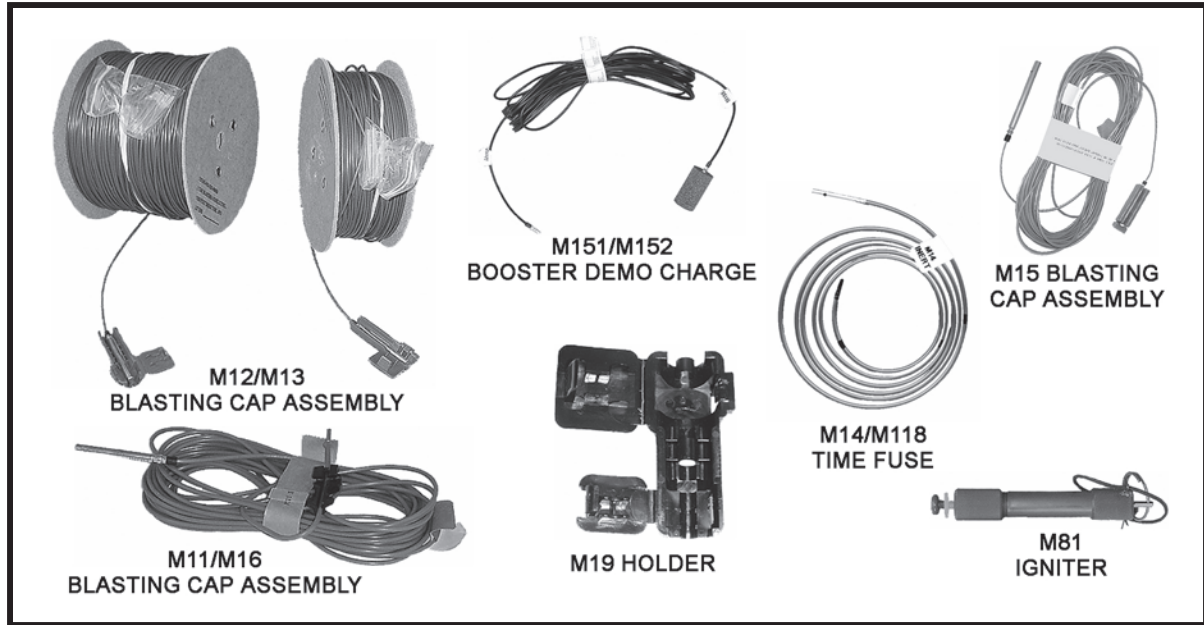
Figure 14-8. MDI components.
