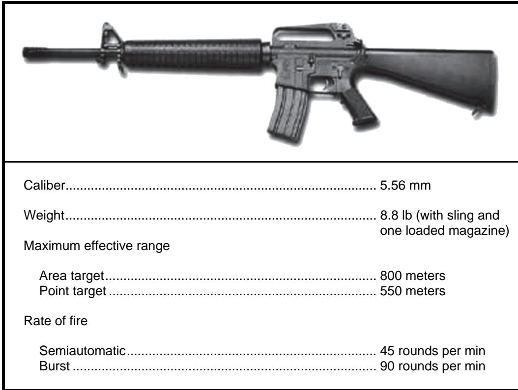
Figure 10-2. M16A2 rifle.
