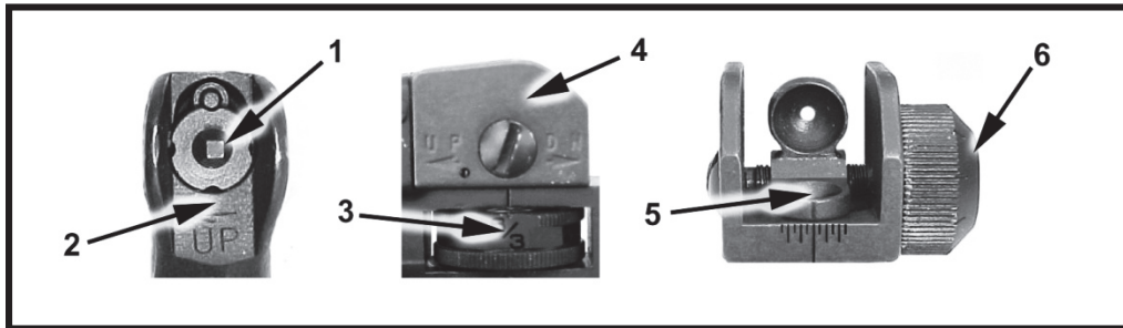
Figure 10-13. M16A2/A3 rifle mechanical zero.
