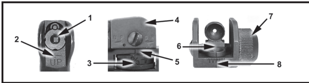
Figure 10-14. M16A4 and M4 carbine rifle mechanical zero.
