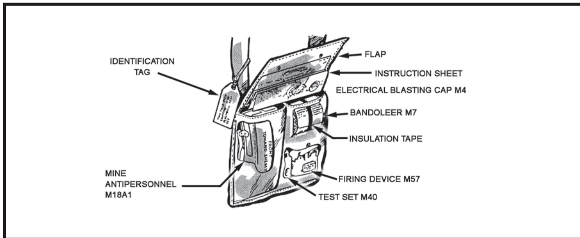
Figure 14-2. M7 bandoleer.
