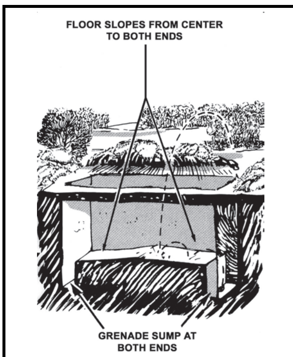
Figure 6-12. Grenade sumps.
