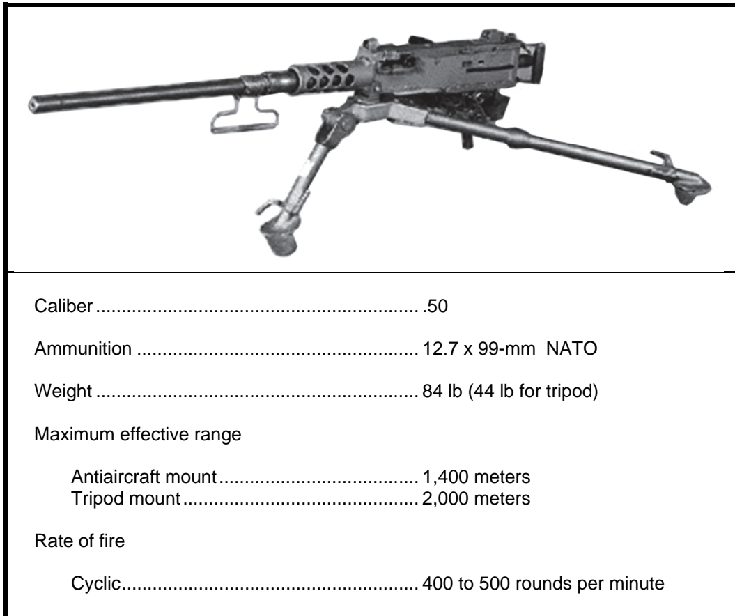
Figure 10-7. M2 .50 caliber machine gun with M3 tripod mount.
