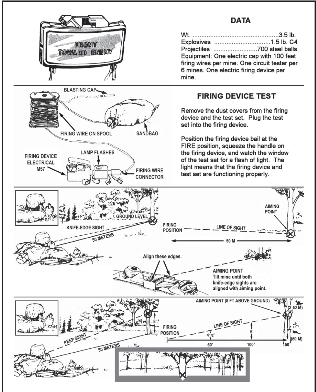
Figure 14-3. M18A1 antipersonnel mine data.
